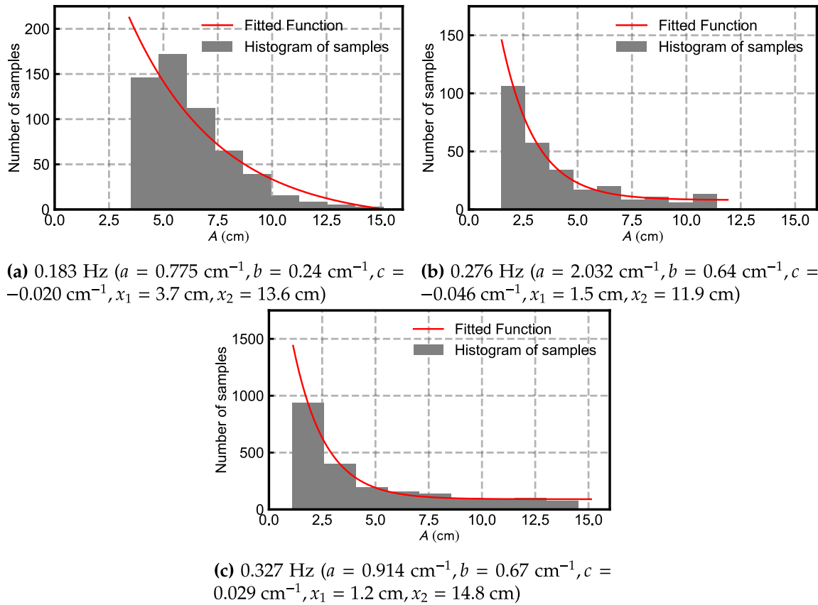
Fig. 6. Distributions of displacement amplitude A .
