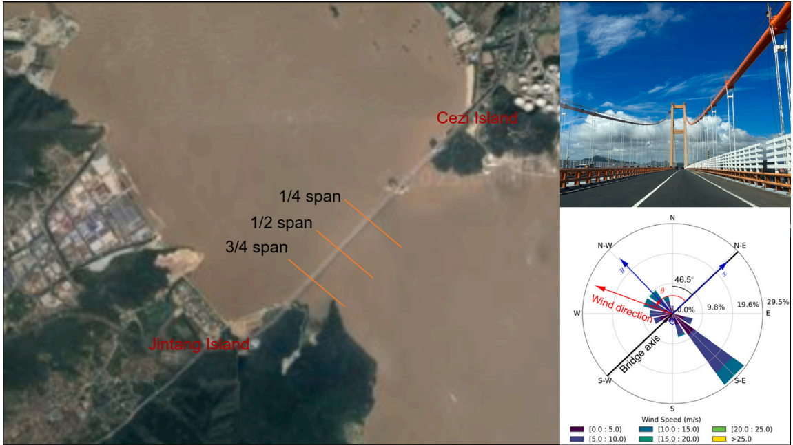
Fig. 2. Location of the investigated bridge.
