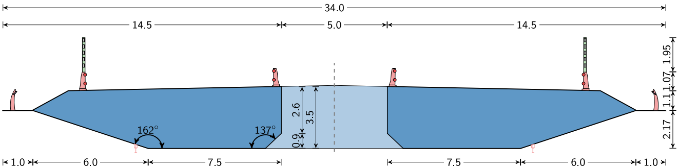
Fig. 3. Bridge Section of the investigated bridge (unit: m).
